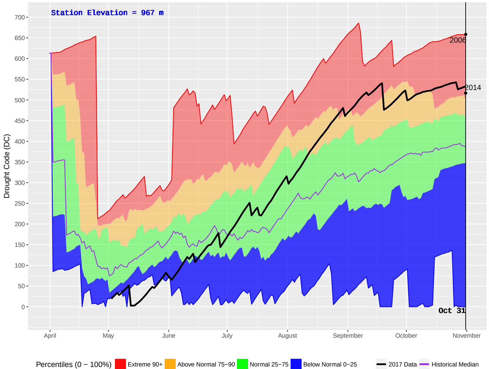
WONOWON (136) : Historical (1990–2016) and Current (2017) Noon Drought Code (DC)
