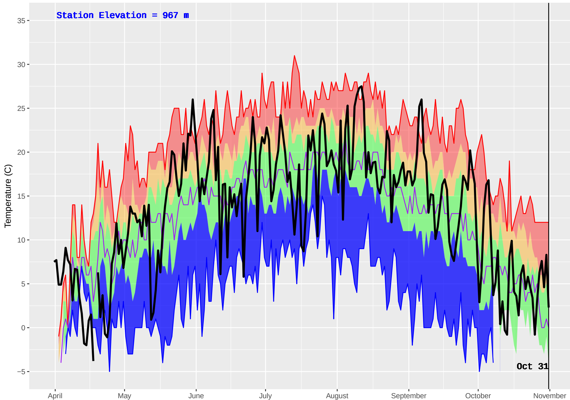
WONOWON (136) : Historical (1990–2016) and Current (2017) Noon Temperature
