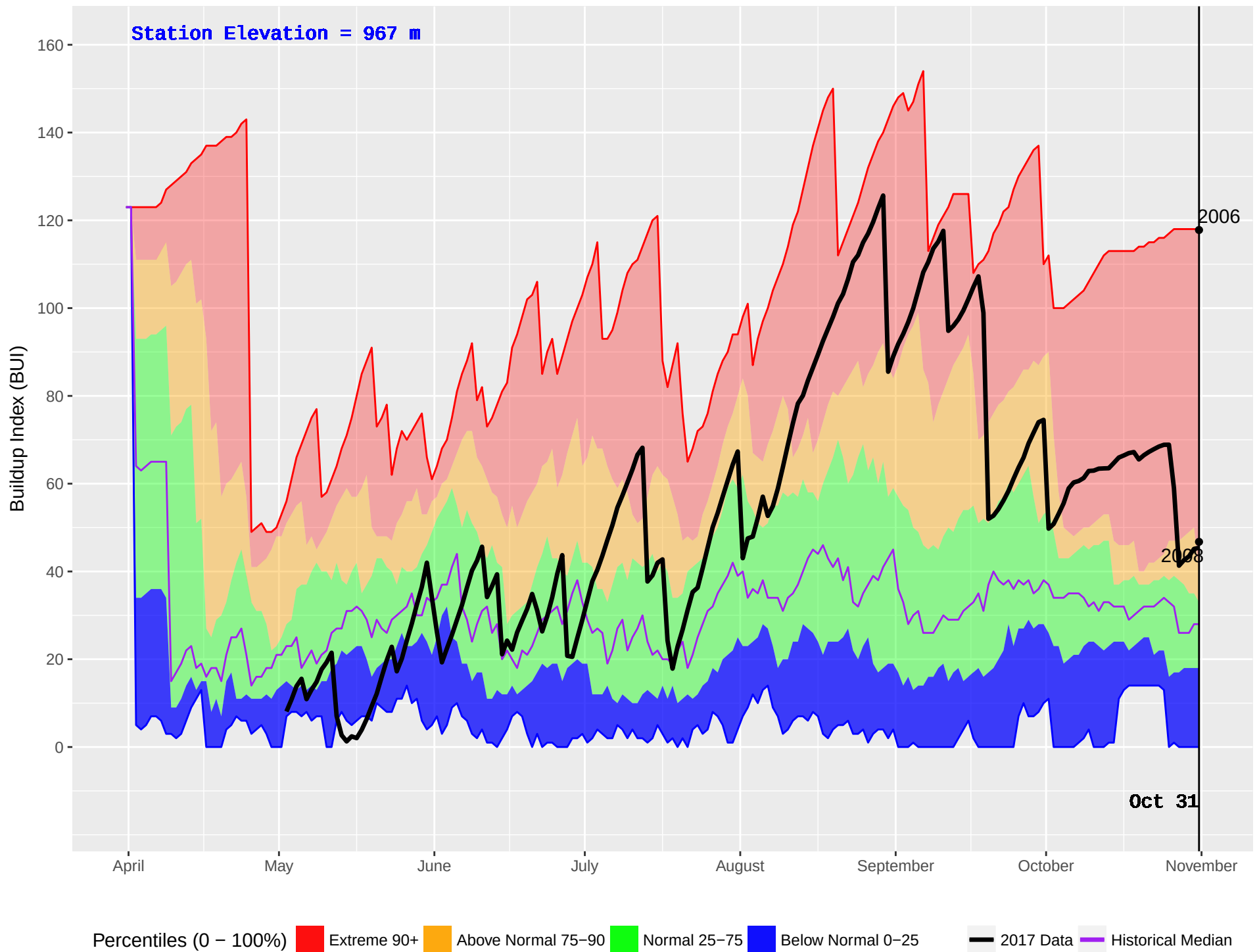
WONOWON (136) : Historical (1990–2016) and Current (2017) Noon Buildup Index (BUI)
